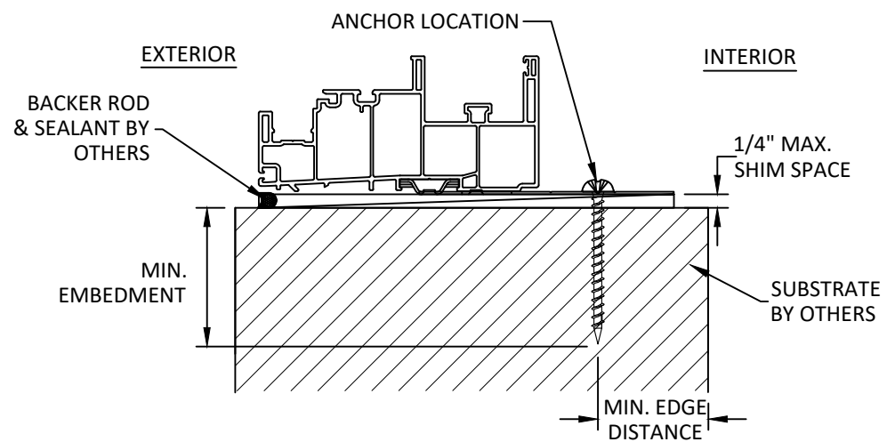
B 10 ANCHOR DETAIL CLIP INSTALLATION SILL
