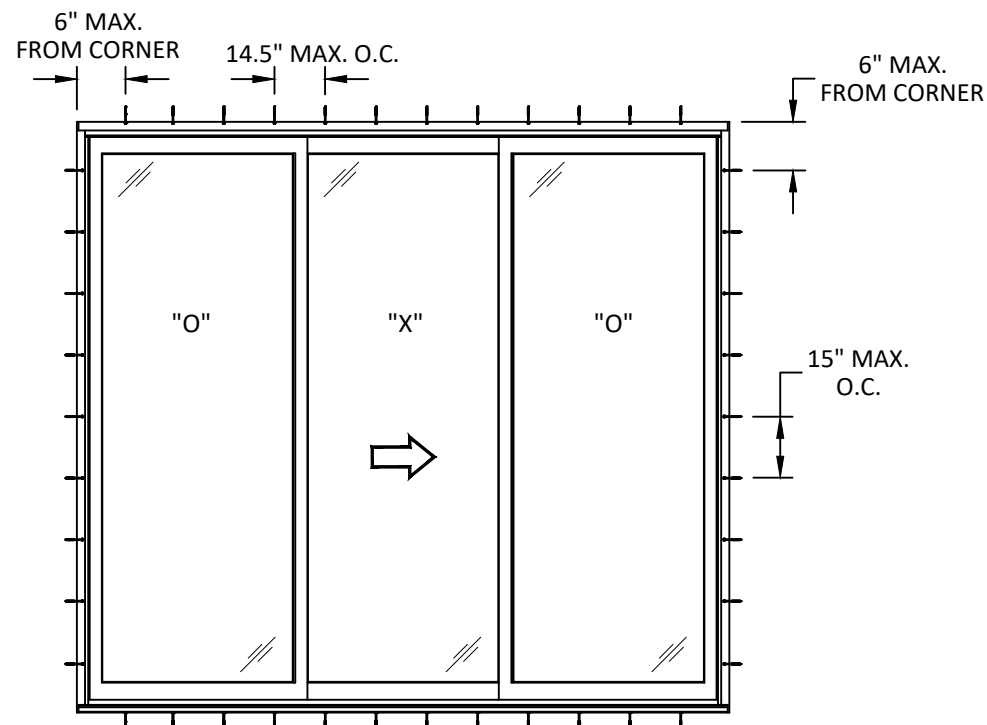
ANCHOR LAYOUT SLIDING DOOR CLIP INSTALLATION
