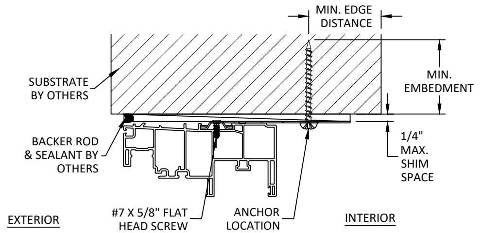
A 10 ANCHOR DETAIL CLIP INSTALLATION HEAD HEAD SHOWN, JAMB SIMILAR
